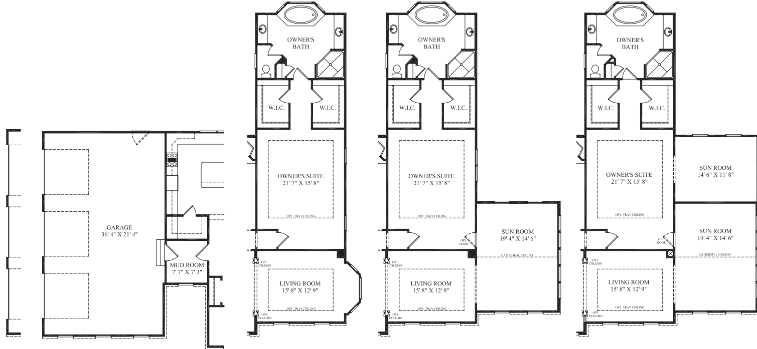
Partial First Floor Plan w/ Opt. 9' Garage Doors Partial First Floor Plan w/ Opt. 3-Car Garage Partial First Floor Plan w/ Opt. Extended Owner's Suite Partial First Floor Plan w/ Opt. Extended Owner's Suite & Opt. Side Sun Room Partial First Floor Plan w/ Opt. Extended Owner's Suite & Opt. Side Sun Room & Opt. Sitting Room
