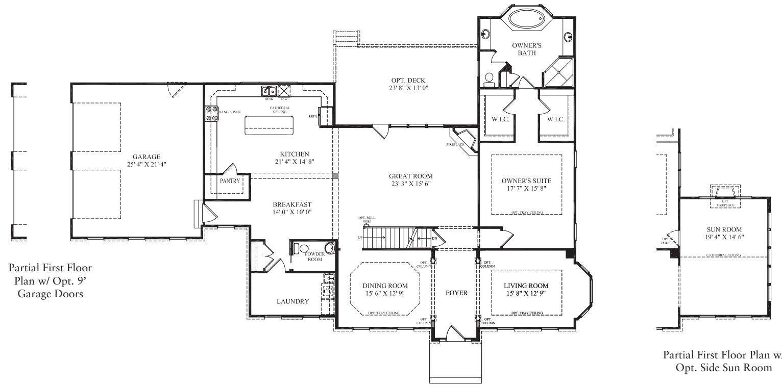
Partial First Floor Plan w/ Opt. 9' Garage Doors Partial First Floor Plan w/ Opt. 3-Car Garage Partial First Floor Plan w/ Opt. Extended Owner's Suite Partial First Floor Plan w/ Opt. Extended Owner's Suite & Opt. Side Sun Room Partial First Floor Plan w/ Opt. Extended Owner's Suite & Opt. Side Sun Room & Opt. Sitting Room
