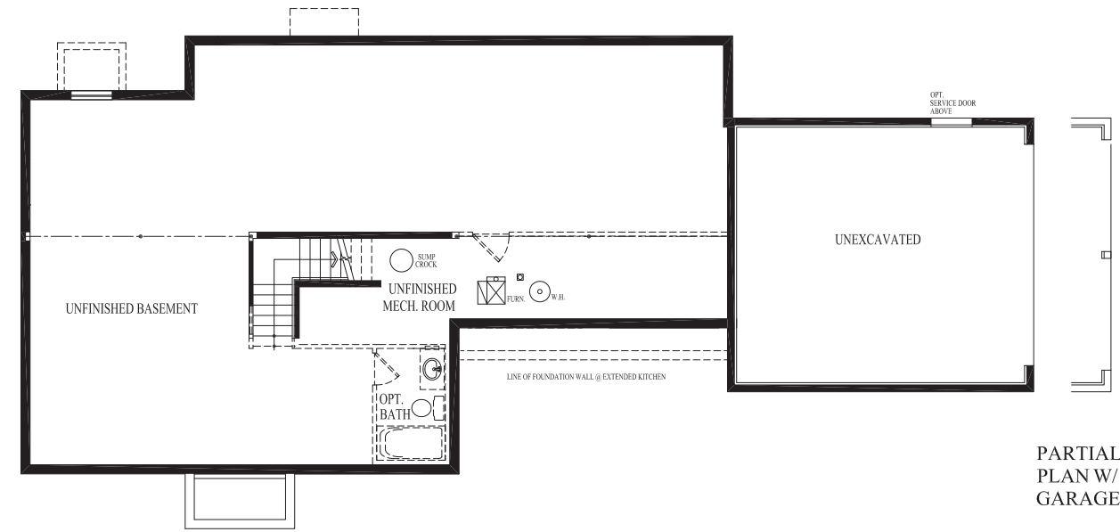
Foundation Plan – Inground Condition
